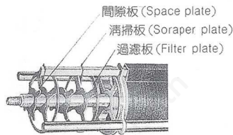
濾板之結構 Construction of a filter plate
