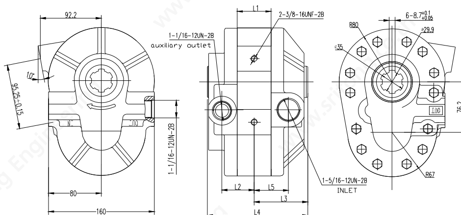
CB-P***LJ42H21SS Installation Dimensions - CB-P***LJ42H21SS
